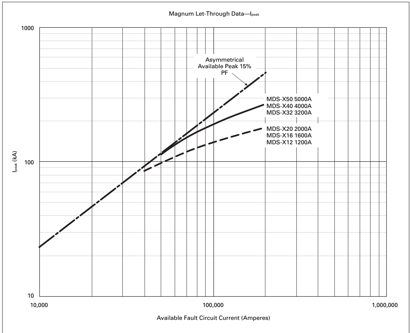
Figure 1. Type Magnum DSX Fuseless Current-Limiting Breakers—Peak Let-Through Curves
