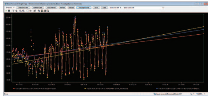
Example of a predictive graph showing the use of historical data and projecting possible future capacity issues. This type of functionality provides the means to automatically be alerted to a capacity problem based on historical data well in advance of an actual problem.
