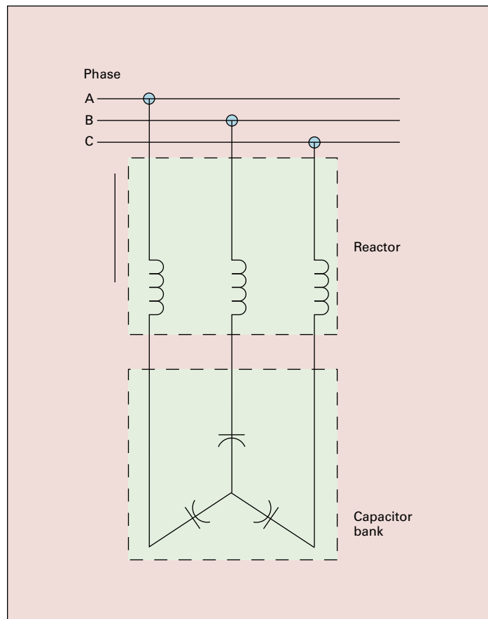
Figure 21. Shunt harmonic filter
