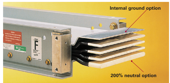
Busway consists of insulated conductors contained within a housing.
